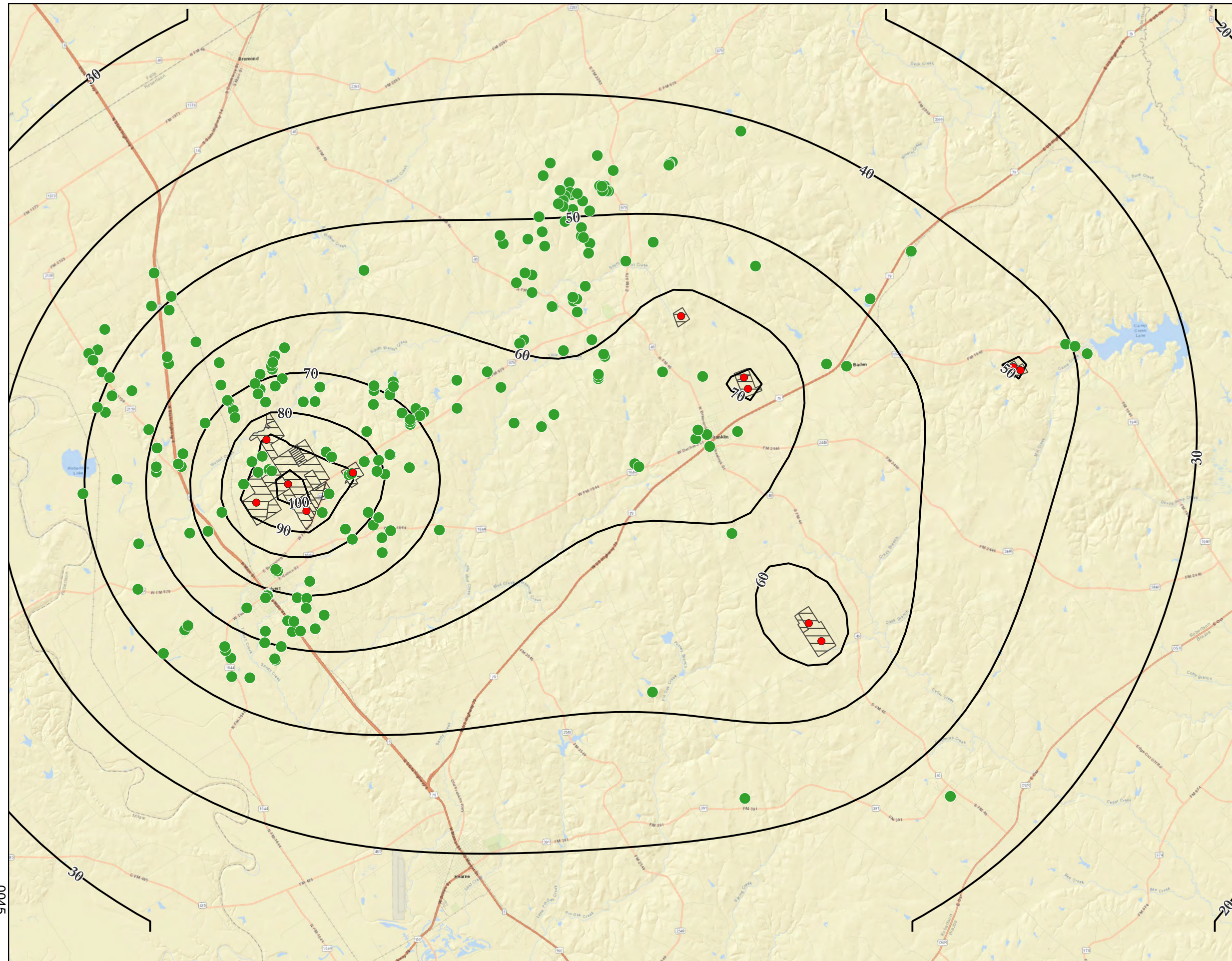
Figure 8: 10-Year Analytical Drawdown Contours
